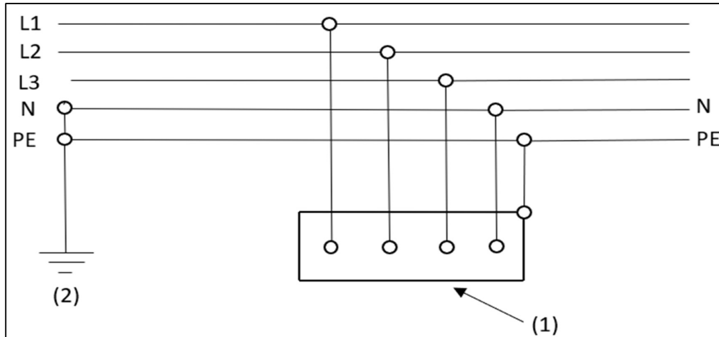
Figure 2.1. Schéma TN-S
