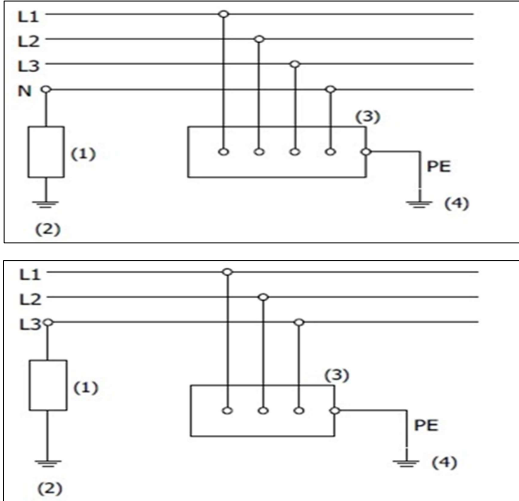
Figure 2.5. Schéma IT
