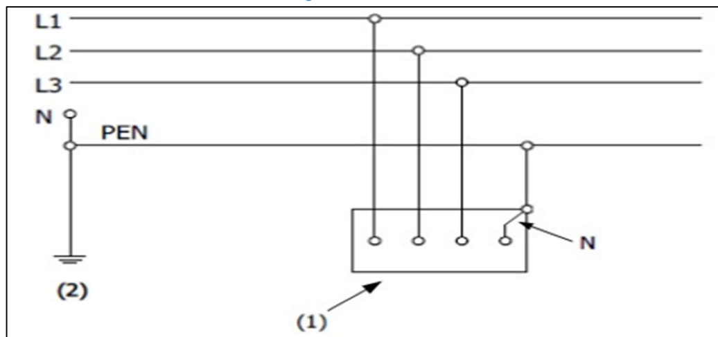
Figure 2.2. Schéma TN-C
