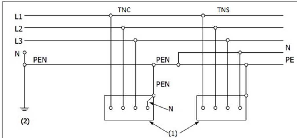
Figure 2.3. Schéma TN-C-S
